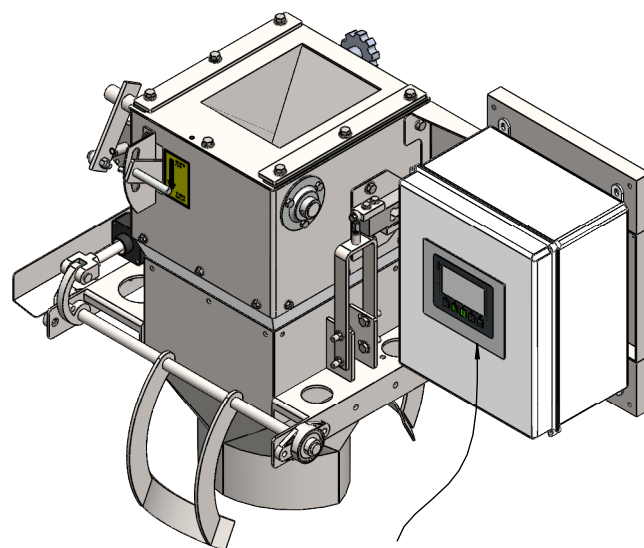
IT1 Scale Controller
